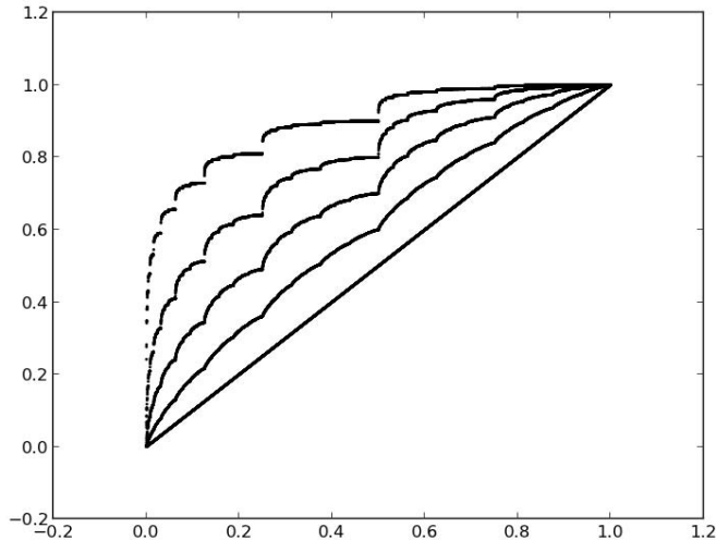
FIGURE 1. Graphs of f_p for p = .1, .2, .3, .4, .5
