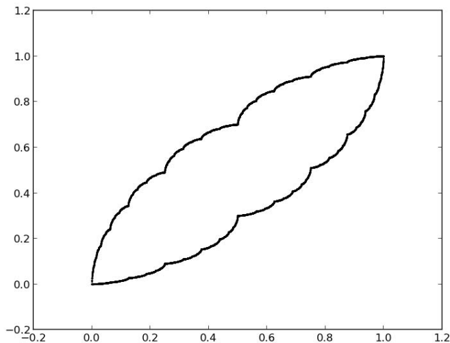
FIGURE 2. Graphs of f_p for p = .3, .7 to illustrate the relation between f_p and f_{1-p} .
