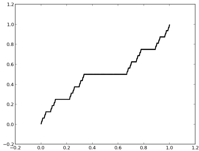
FIGURE 3. The Devil's staircase.
