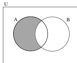
Set Difference ( A - B ):
