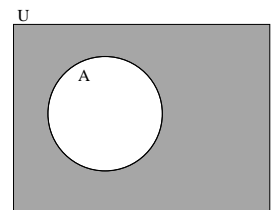
Set Complement \bar{A} :
