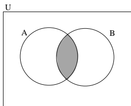
Set Intersection ( A \cap B ):
