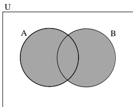
Set Union ( A \cup B ):
