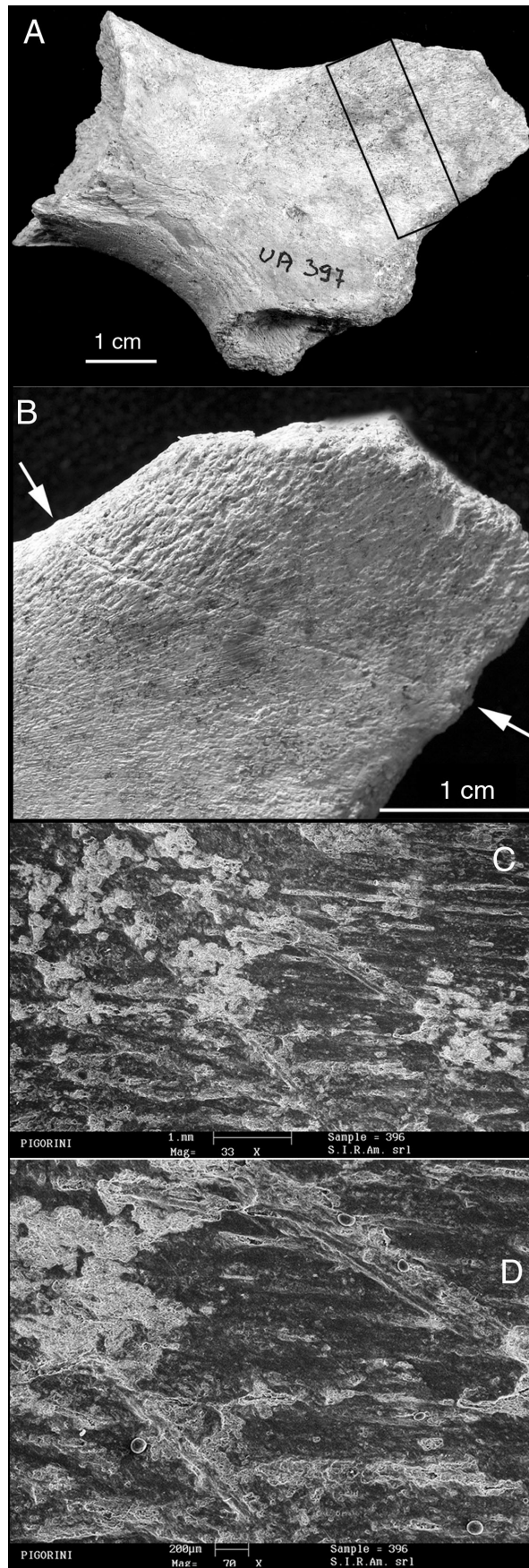
Fig. 6 - UA-397. A) undetermined middle size mammal coxal fragment; B) lithic-tool cutmarks; C-D) SEM details of rectilinear, sub-parallel striae; numerous secondary striae are noticeable.
