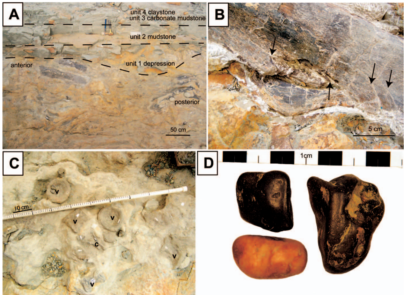
FIGURE 6 —Tooth-damaged and trampled bones in unit 1. (A) Depression in unit 1 with scapulae and pubic bone. Unit contacts are indicated by dashed lines. (B) Tooth damage in the form of V-shaped grooves on scapula indicated by arrows. (C) Caudal vertebrae (v) vertically impressed into unit 1 with adjacent chevron (c) and other horizontal vertebrae. (D) Three presumed gastroliths found near pelvic girdle elements.
