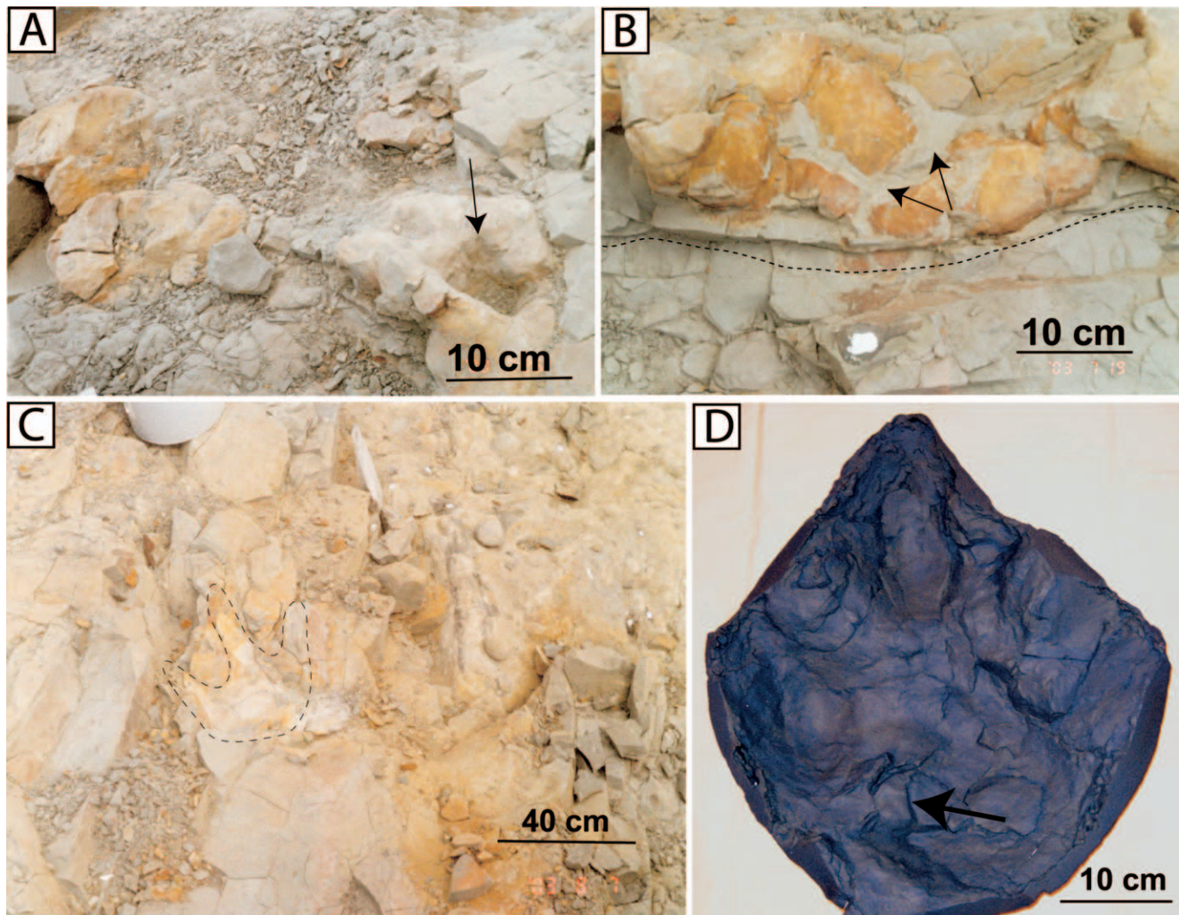
FIGURE 4 —Identification of tracks in unit 3 sediments. (A) Unit 3 carbonate mudstone immediately above track. Note the collapse feature indicated by arrow. (B) Loading under carbonate mudstone. Claystone inside carbonate mudstone is shown by arrows. (C) Tridactyl track on unit 2 (dashed line) before casting. (D) Cast of tridactyl track from top of unit 2. Arrow indicates pullup; specimen WDC-SI-696.
