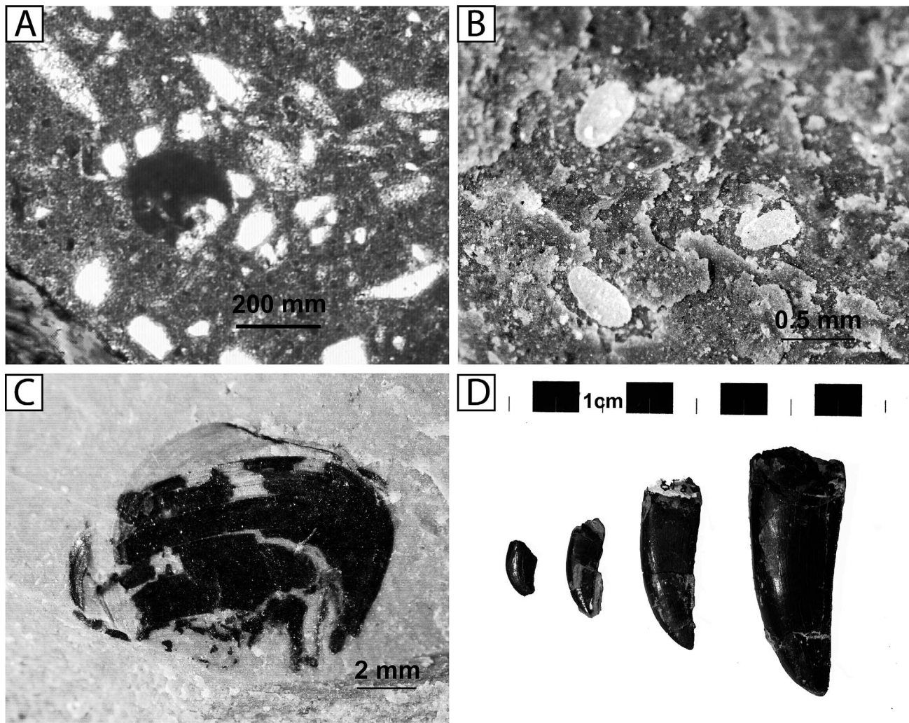
FIGURE 5 —Fossils from units 1 and 4. (A) Bioclasts in unit 1; XPL. (B) Ostracodes in unit 4; specimen WDC-SI-837. (C) Conchostracan from unit 4, specimen WDC-SI-838. (D) Range of sizes of theropod teeth from SI quarry; left to right: WDC-SI-659, WDC-SI-698, WDC-SI-748, WDC-SI-754.
