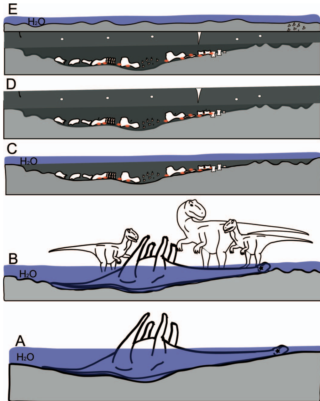
FIGURE 10 —Sequence of events at SI quarry. (A) Dead juvenile Camarasaurus in shallow water. (B) Allosaurids scavenging the decaying carcass. (C) Burial after scavenging and subsequent barite precipitation (D) Weak paleosol development after regression of water. (E) Return of subaqueous conditions followed by the development of trampled carbonate mud and second theropod tooth-bone assemblage.
