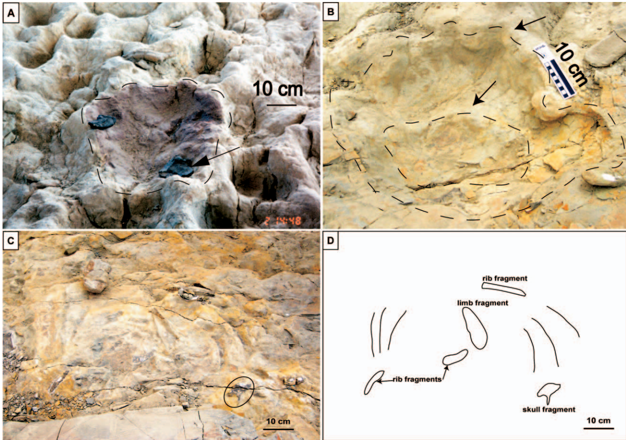
FIGURE 7 —Bioturbation in unit 1. (A) Oblique view of a large track cutting across tracks that extend deeper into the trampled surface. Cast of small flattened caudal vertebrae in approximate original position in the track is indicated by arrow. (B) Juvenile sauropod track with heel-pad impression indicated by dashed lines. Arrows show pushups in direction of movement (east). (C) Tridactyl, clay-filled V-shaped grooves at south end of the depression in unit 1. Skull fragment is circled. (D) Diagram of V-shaped grooves and associated bones.
