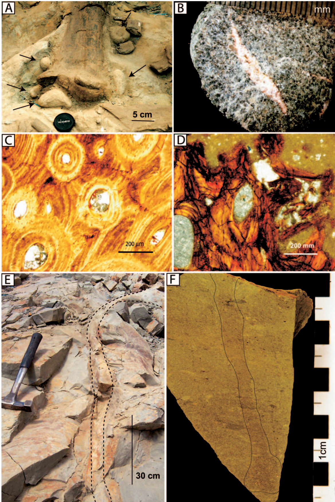
FIGURE 3 —Features in two apparently homogeneous units. (A) Barite nodules formed around limb bones in unit 1. (B) Granular textured barite nodule with sparry calcite in center. (C) Permineralized bone from unit 1 showing no compaction features; cross-polarized light (XPL). (D) Weathered bone fragment in micritic carbonate from unit 2, XPL. (E) Desiccation crack (dashed lines) in unit 2. (F) Vertical burrow (dotted line) from unit 2.
